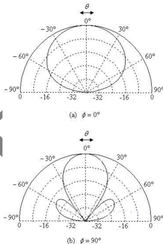
Fig 4. Normalized Radiation Pattern for Microstrip (Patch) Antenna.
