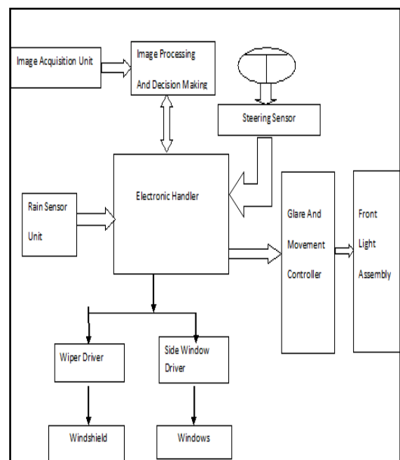
Fig.2. block diagram of the implemented system
