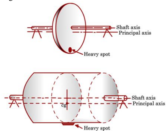
Fig.1 Statically Unbalanced System
