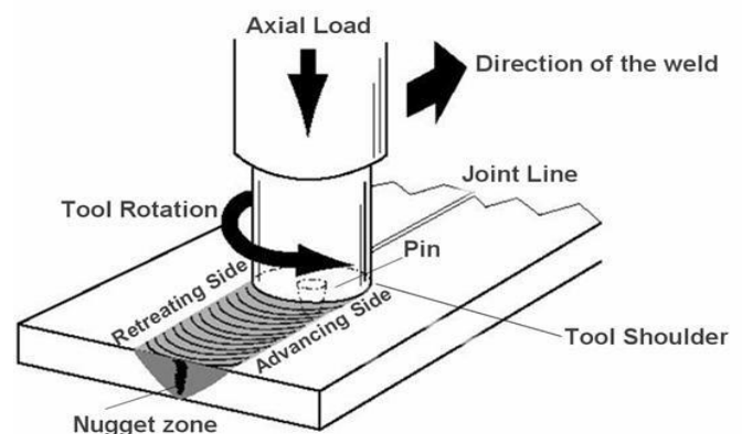
Fig-1: Schematic of Friction Stir Welding
