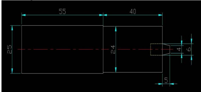
Fig-2: FSW Tool Design
