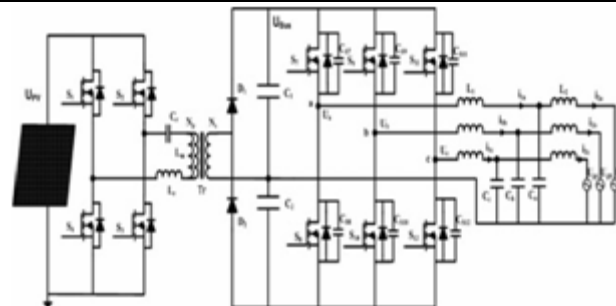
Fig. 1 Two-stage three-phase four-wire grid-tie inverter system.
