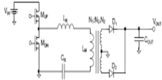
Fig.3.4. Scheme of a single module LLC resonant converter.
