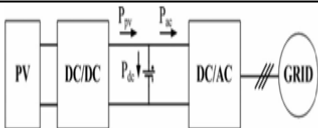
Fig. 15. Simplified block diagram of two-stage MIC
