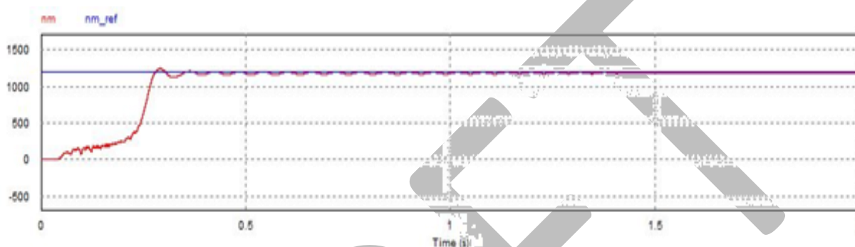
Fig. 10. Speed Response of V/F control for ZSI fed IM Drive (1200RPM)
