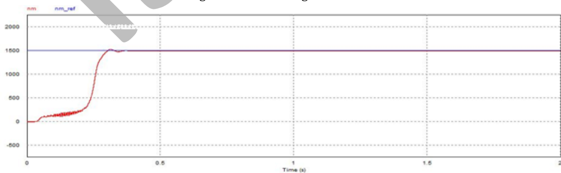
Fig. 8. Reference speed and actual speed plot of ZSI drive
