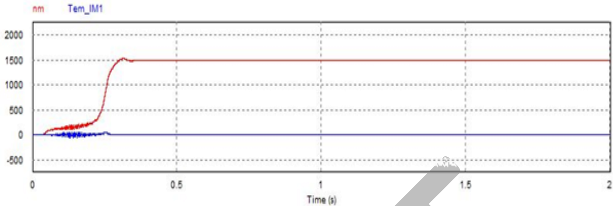
Fig. 5. Speed torque waveform of ZSI fed drive
