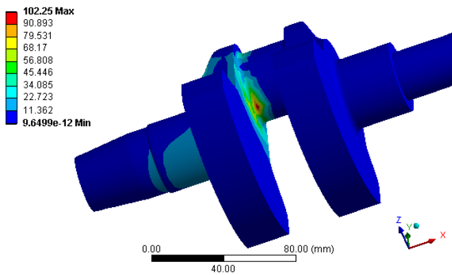
Fig.5 Von Misses Stress
