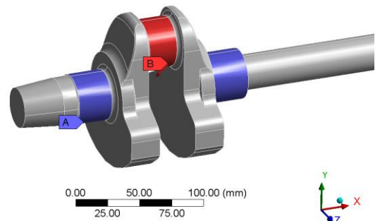
Fig.4 Boundary conditions for crankshaft
