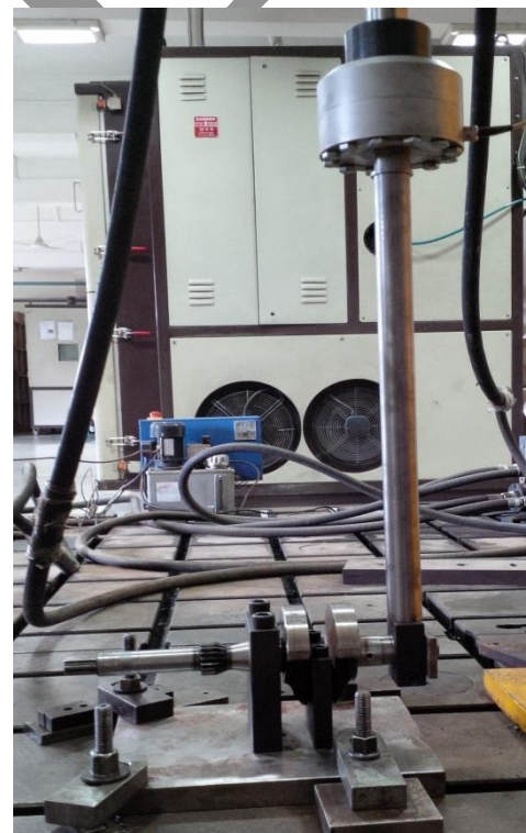
Fig.8 Experimental Set-up
