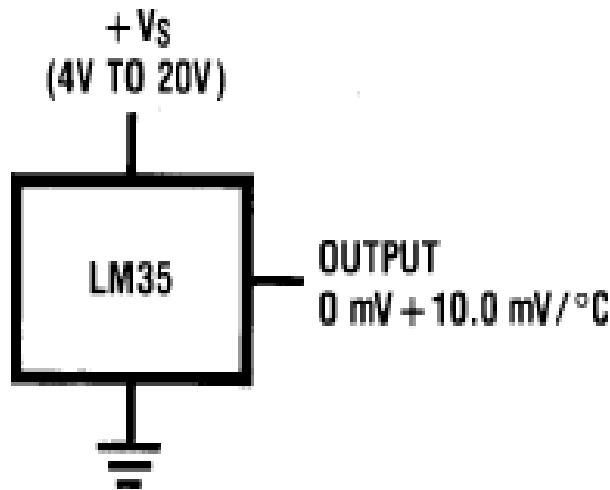
Figure 4 Basic Centigrade Temperature Sensor
