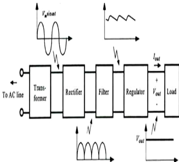
Figure 2 Components of a typical linear power system
